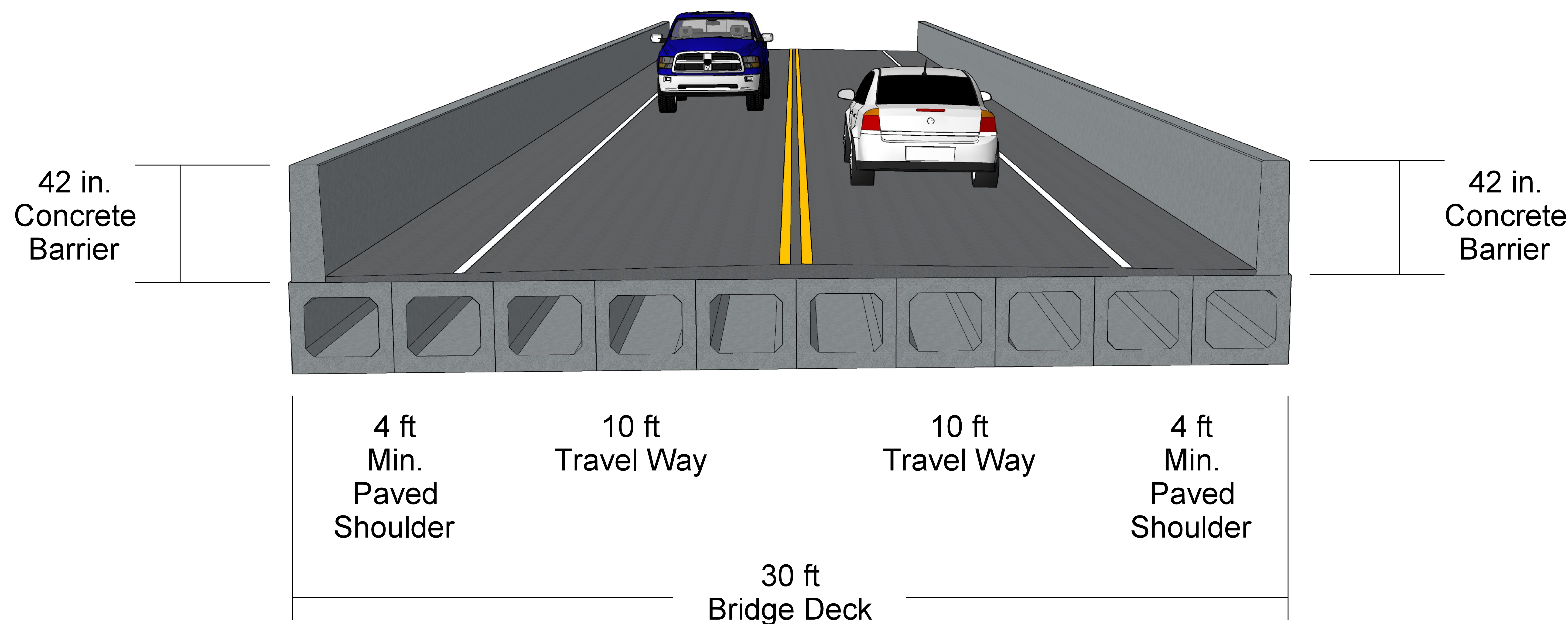
BRIDGE DECK CROSS SECTION
